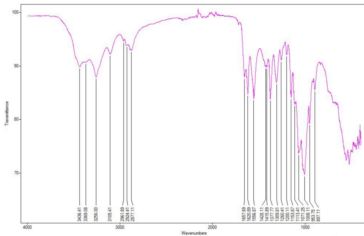
Figure 2: FTIR Spectra of Prawn Chitosan (Procedure B 1 )
