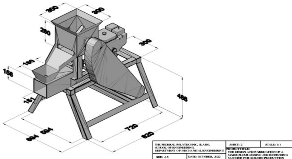
Fig. 2: Isometric View of Kokoro Pasta Extruding Machine
