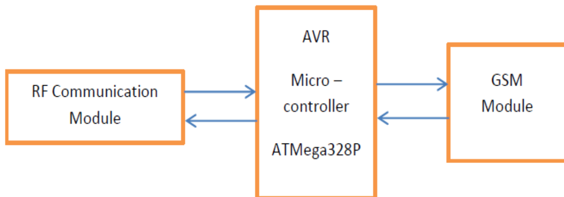
Figure 3: Fire signal receiving block diagram
