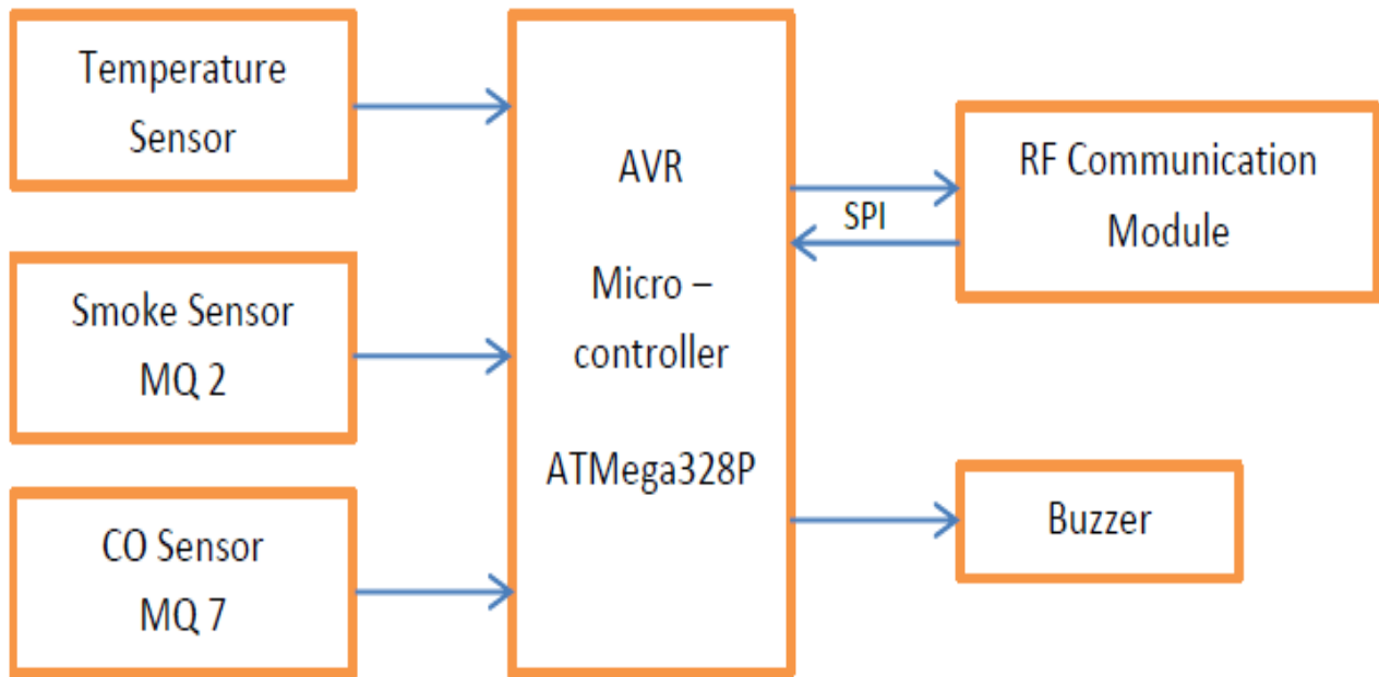
Figure 2: Fire sensing node block diagram
