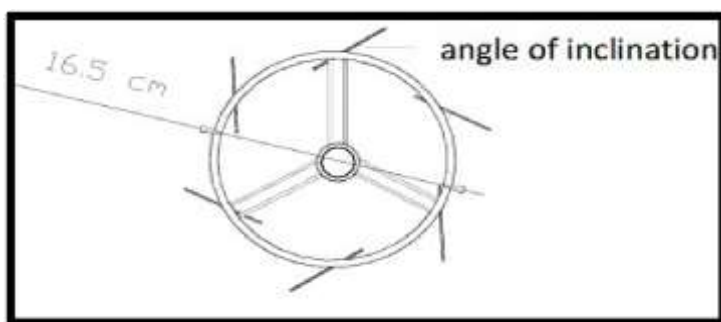
Figure 2: Weeding Frame Diameter Specification and Blade Inclination
